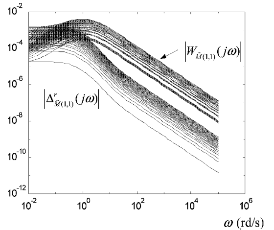
Fig. 3 Upper bound on magnitudes of perturbations for example 1.
